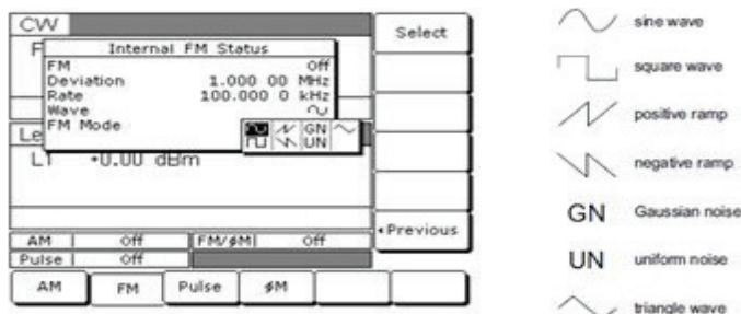
Figure 2. MG3690C Series of Signal Generators Waveforms
